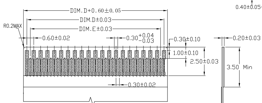
RECOMMENDED FPC DIMENSIONS
